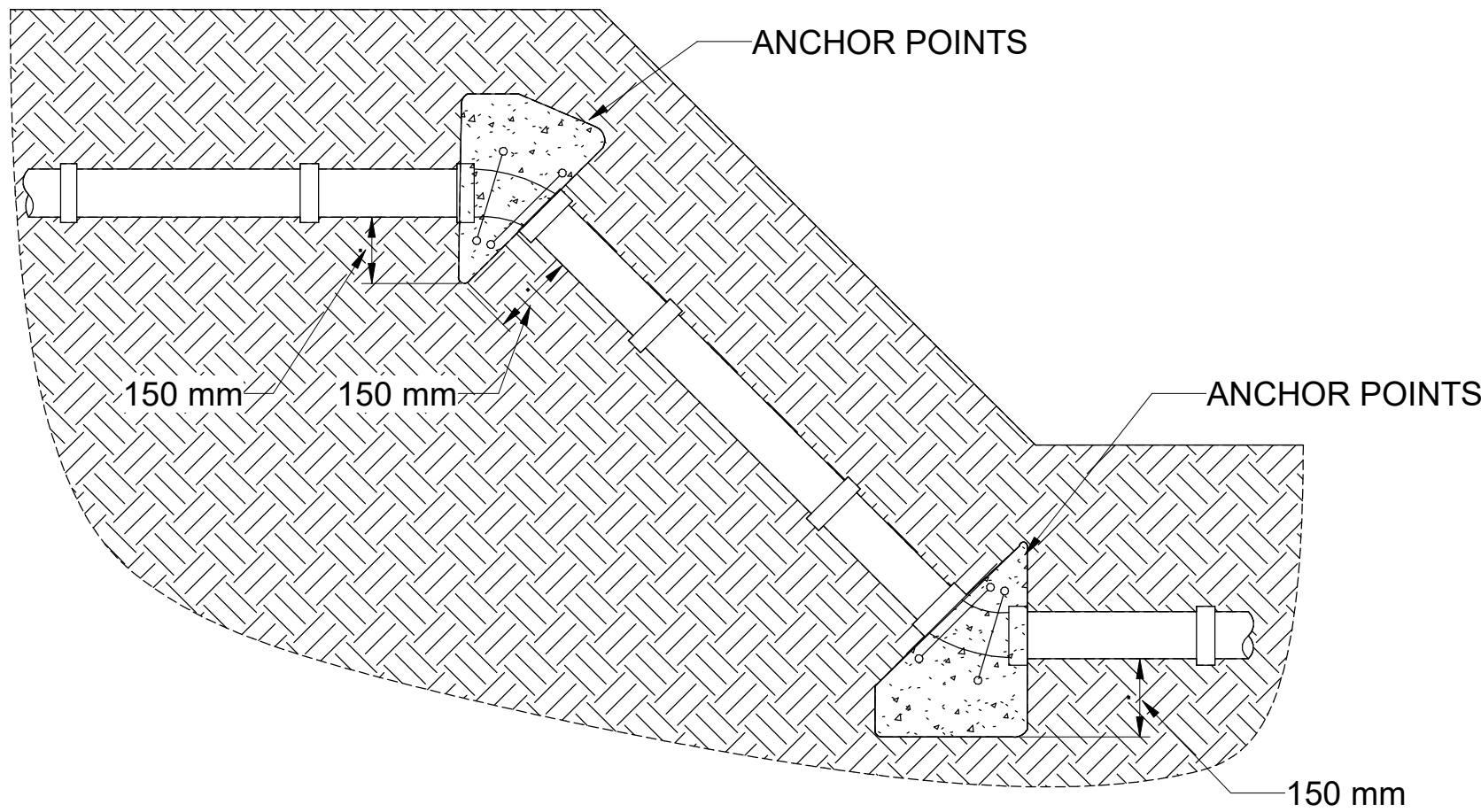
45° JUMP UP DETAIL NTS
