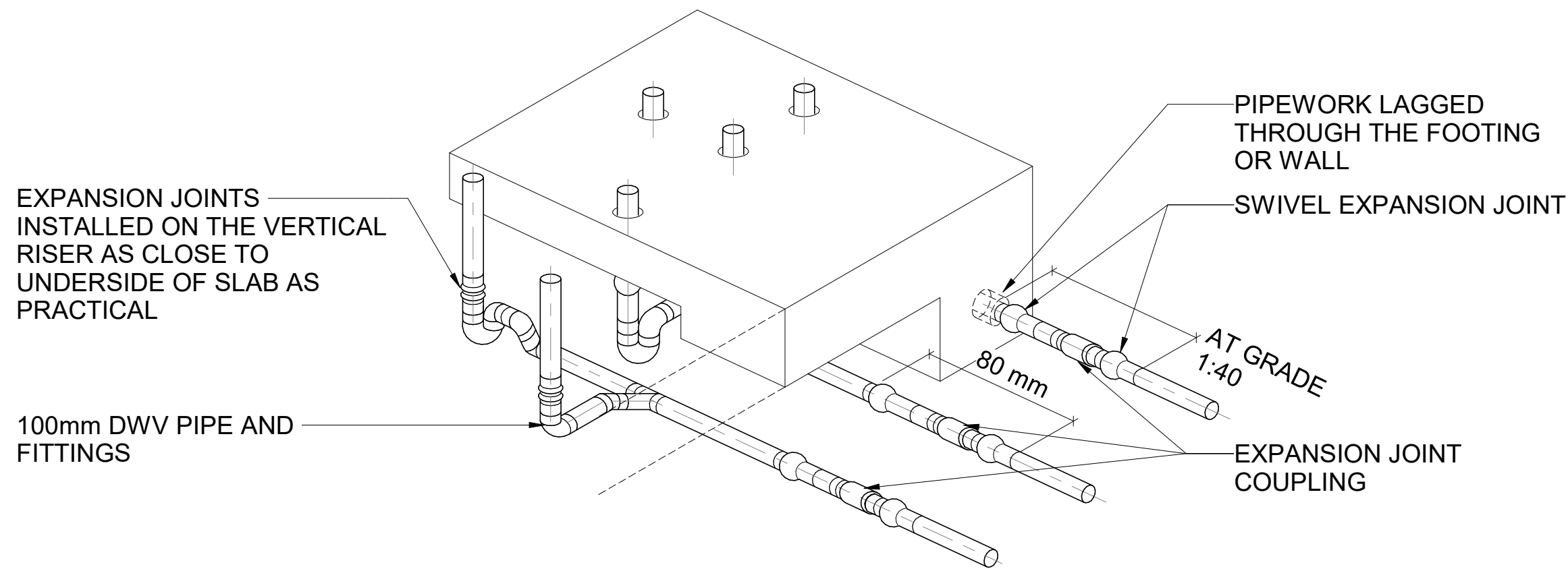
EXPANSION JOINT DETAIL NTS
