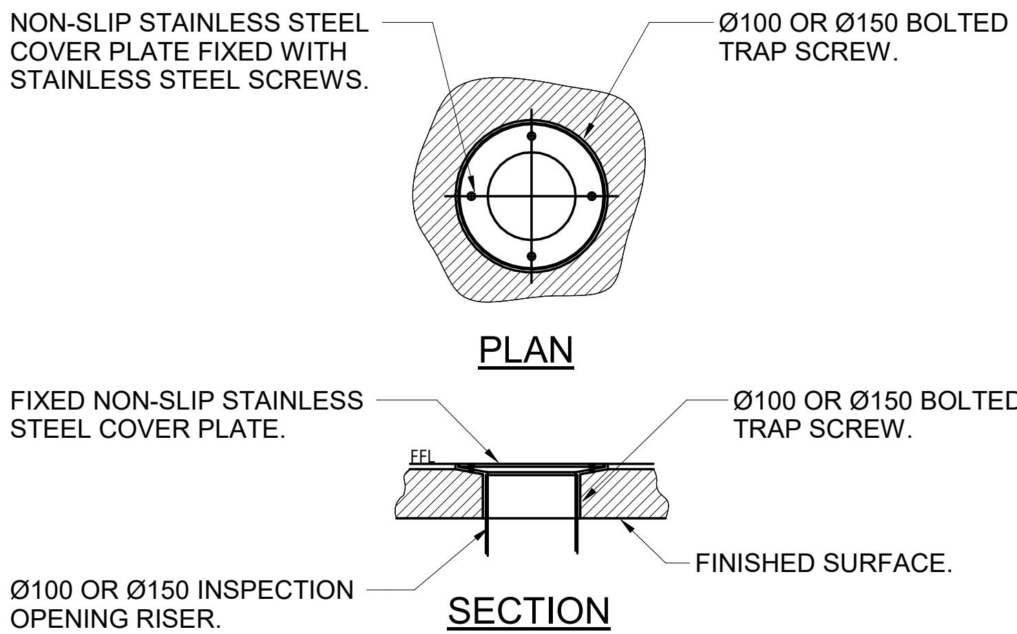
INSPECTION OPENING - NON-SLIP INTERNAL NTS
