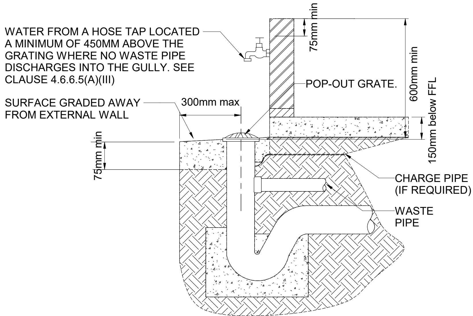
OVERFLOW RELIEF GULLY NTS
