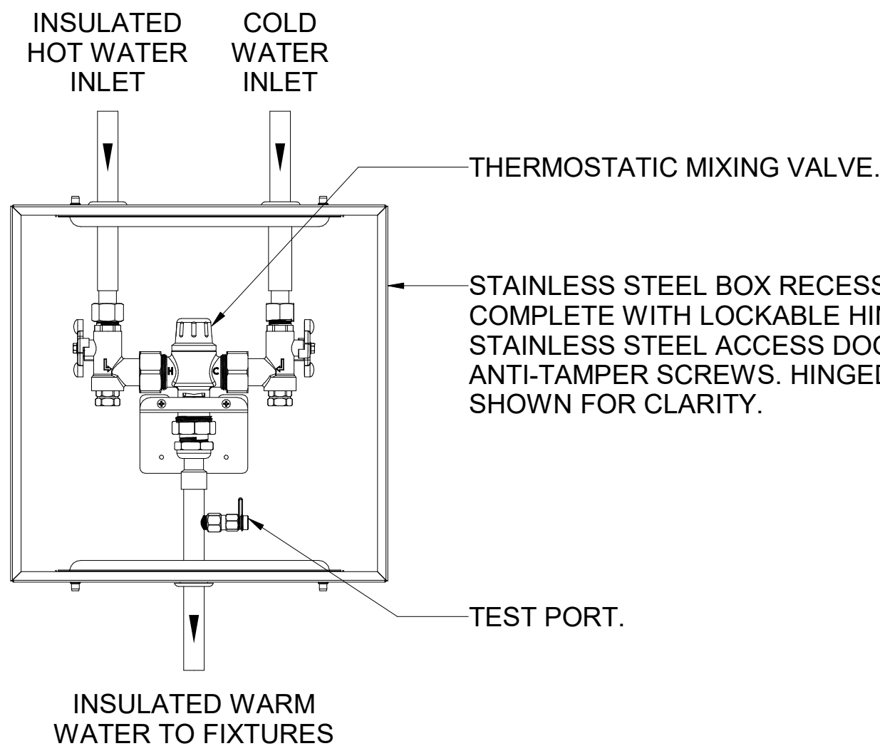
TMV IN WALL BOX NTS
