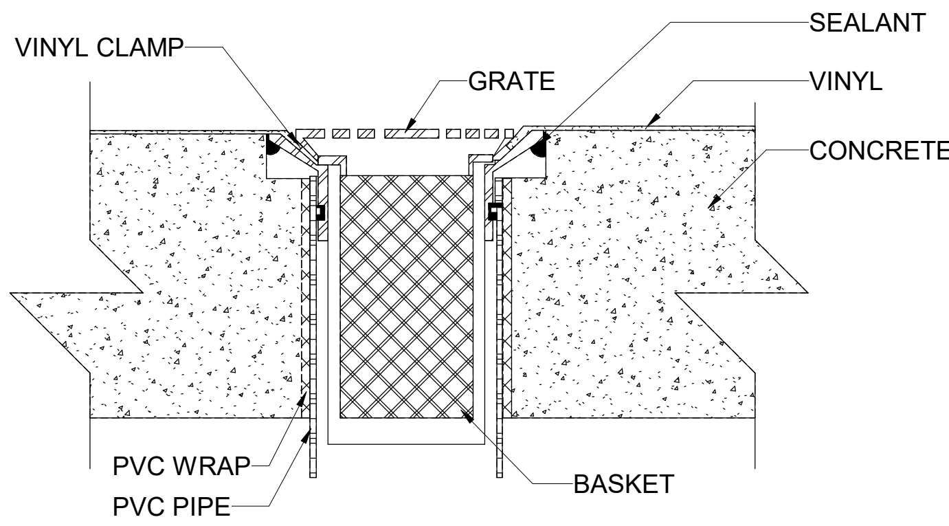
FLOOR/ BASKET WASTE DETAIL NTS
