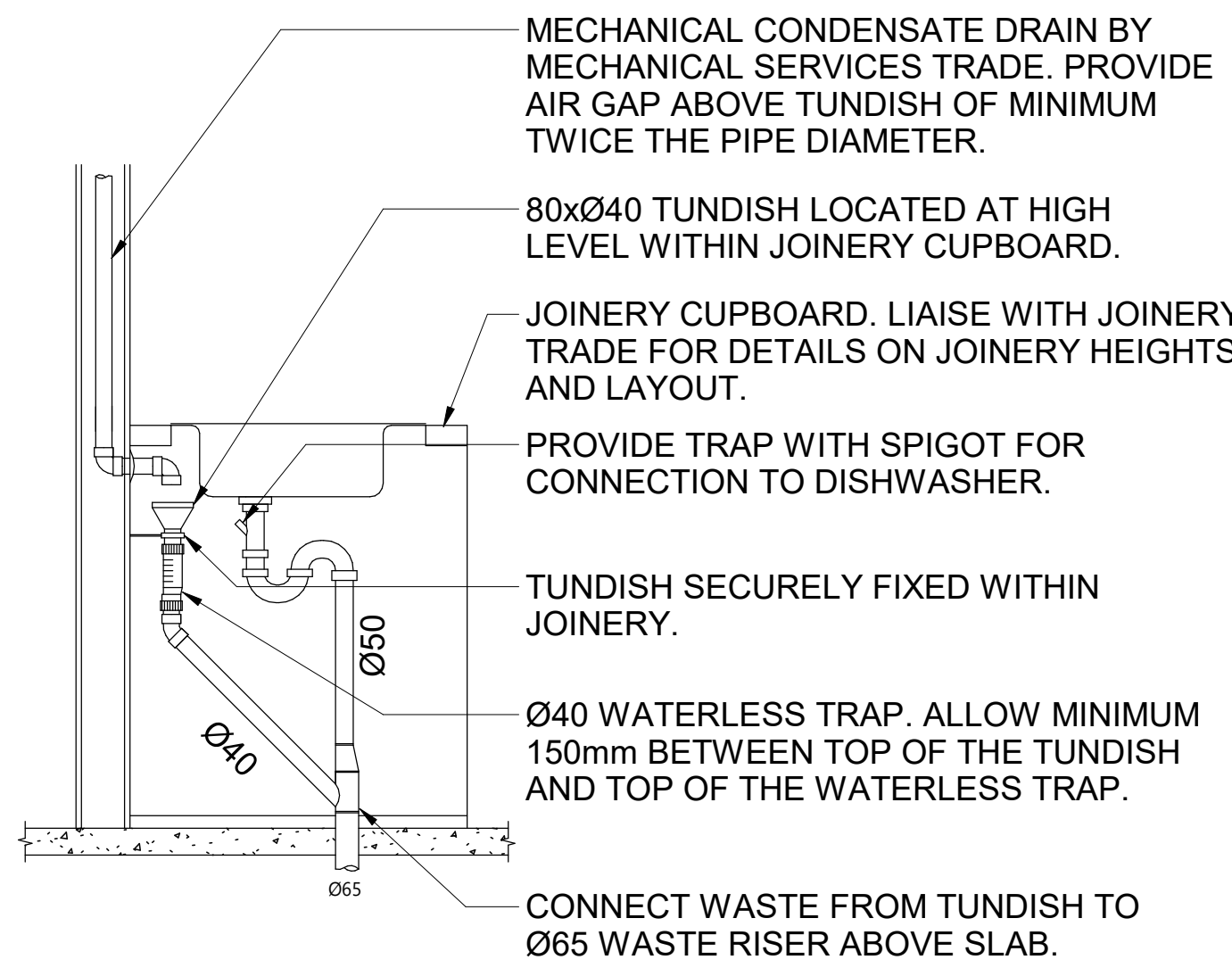
UNDERBENCH TUNDISH FOR A/C DISCHARGE NTS
