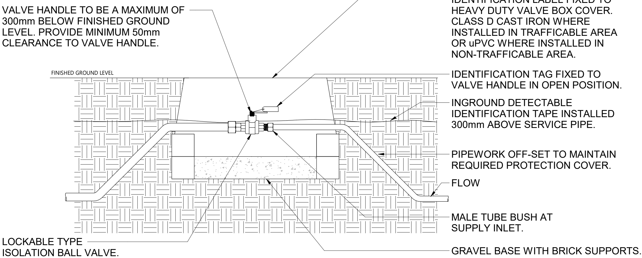
INGROUND ISOLATION VALVE BOX NTS
