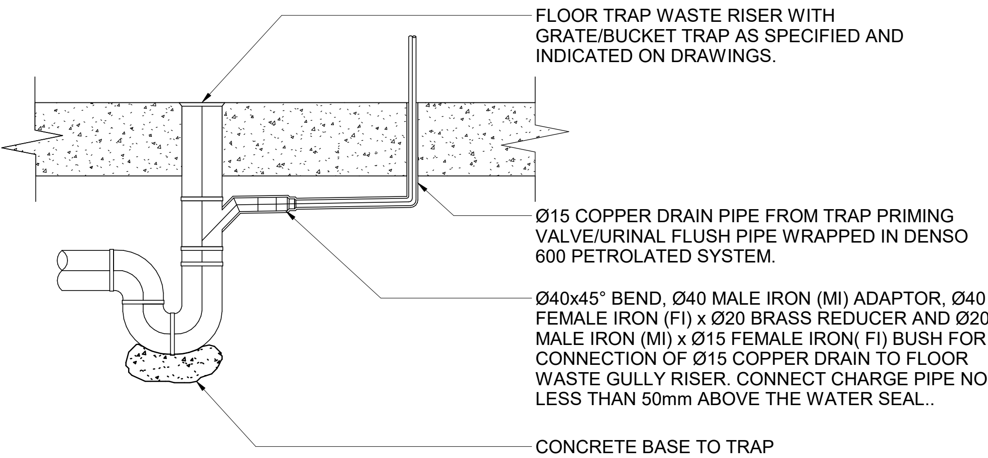
CHARGE LINE TO FLOOR WASTE NTS
